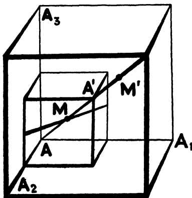
FIG. 15.—The centers of inversion of space-groups O_h^m .
